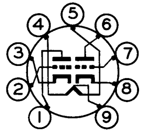
RETMA 9A BOTTOM VIEW
