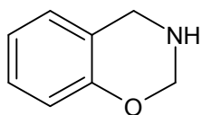
3,4-dihydro-2H-1,3-benzoxazine
