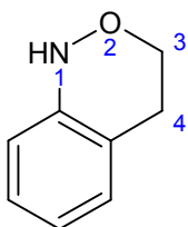
3,4-dihydro-1H-2,1-benzoxazine
