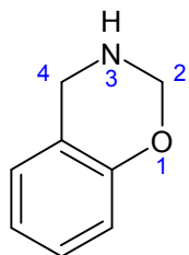
3,4-dihydro-2H-1,3-benzoxazine
