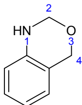
1,4-dihydro-2H-3,1-benzoxazine
