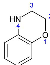
3,4-dihydro-2H-1,4-benzoxazine
