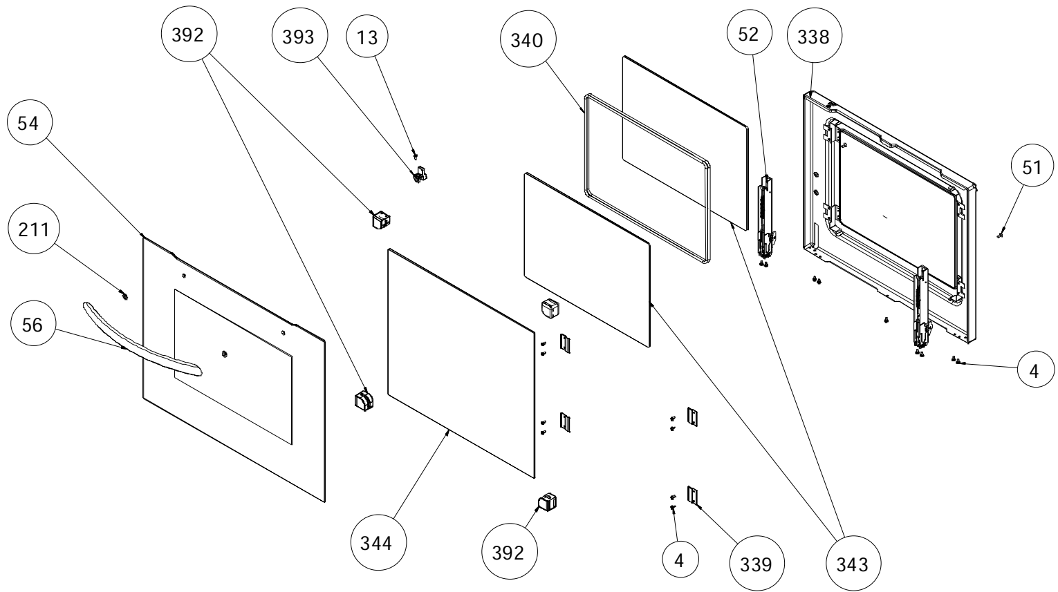
OVEN DOOR ASSEMBLY (OUTER & INNER) (POSITION NO 378)
