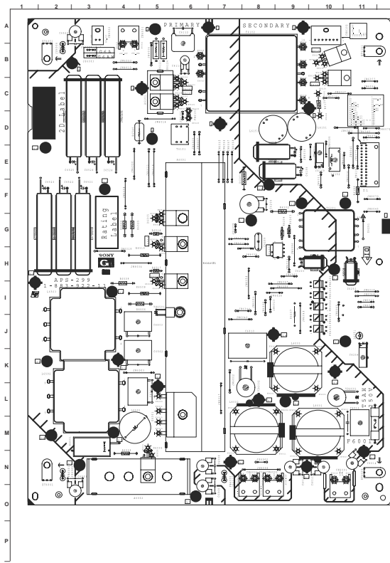
G6 POWER COMPONENT SIDE (KDL-55HX820 ONLY)
