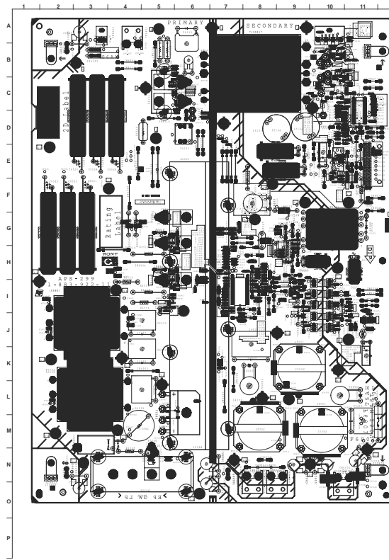
G6 POWER CONDUCTOR SIDE (KDL-55HX820 ONLY)
