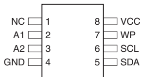
8-lead dBGA2
