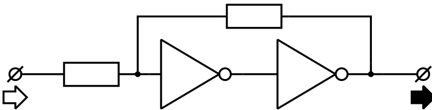
Trigger de Schmitt
