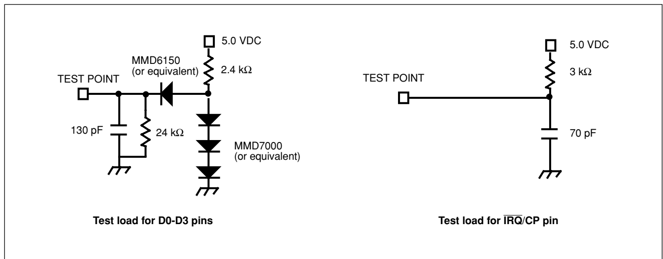
Figure 14 - Test Circuit
