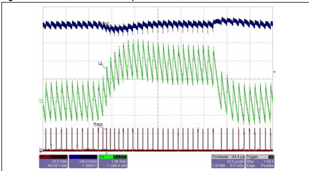
Figure 23. OUT1 load transient response
