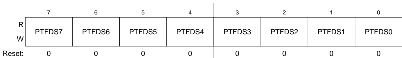
Figure 6-38. Drive Strength Selection for Port F Register (PTFDS)
