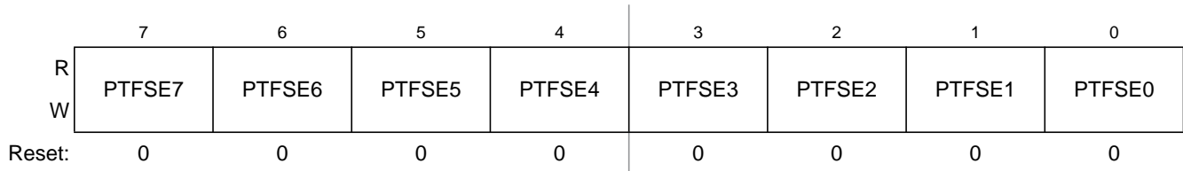
Figure 6-37. Slew Rate Enable for Port F Register (PTFSE)
