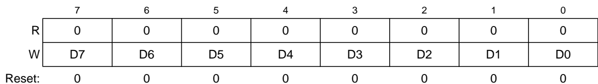
Figure 4-9. Linear Address Pointer Add Byte Register (LAPAB)
