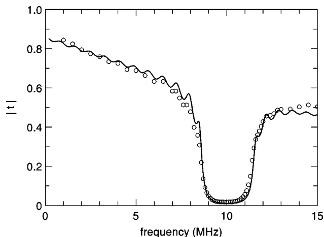
FIG. 1. Transmission coefficient of the electric field through a coaxial photonic crystal with 12 unit cells. The solid line is the expected transmission based on measured system parameters (no adjustments made).
