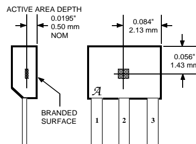
Dwg. MH-011-3D
