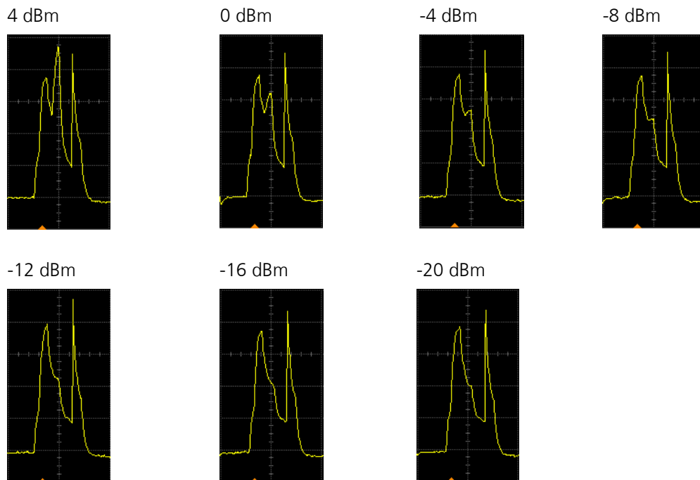
Figure 7: Typical peak current consumption profile (with DCDC ON) during connection event in slave mode versus TX PWR.
