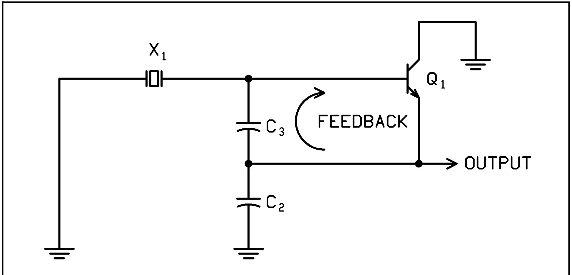
FIGURE 16: COLPITTS CRYSTAL OSCILLATOR
