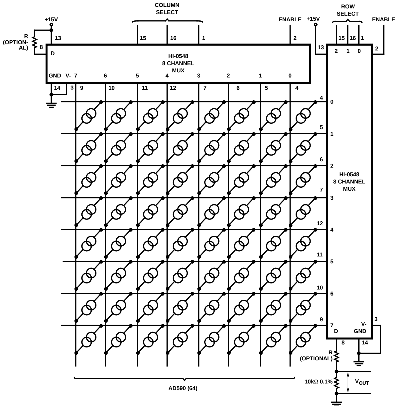
FIGURE 17. MULTIPLEXING SENSORS
