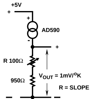
FIGURE 2. SLOPE TRIMMING
