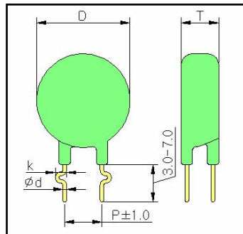
Out Side kinked cutting Type
