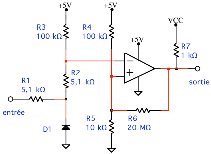
Zéro-crossing detector, single supply
