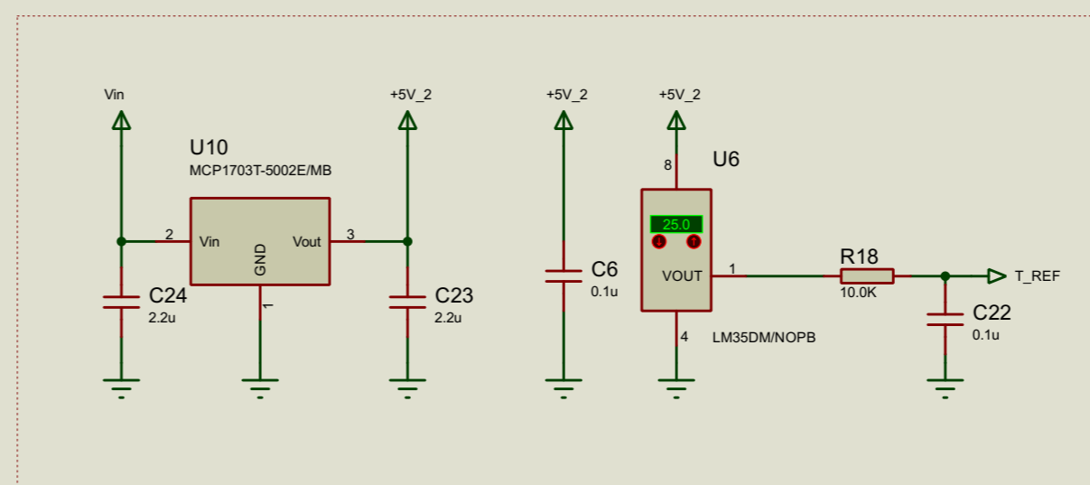
Cold junction
