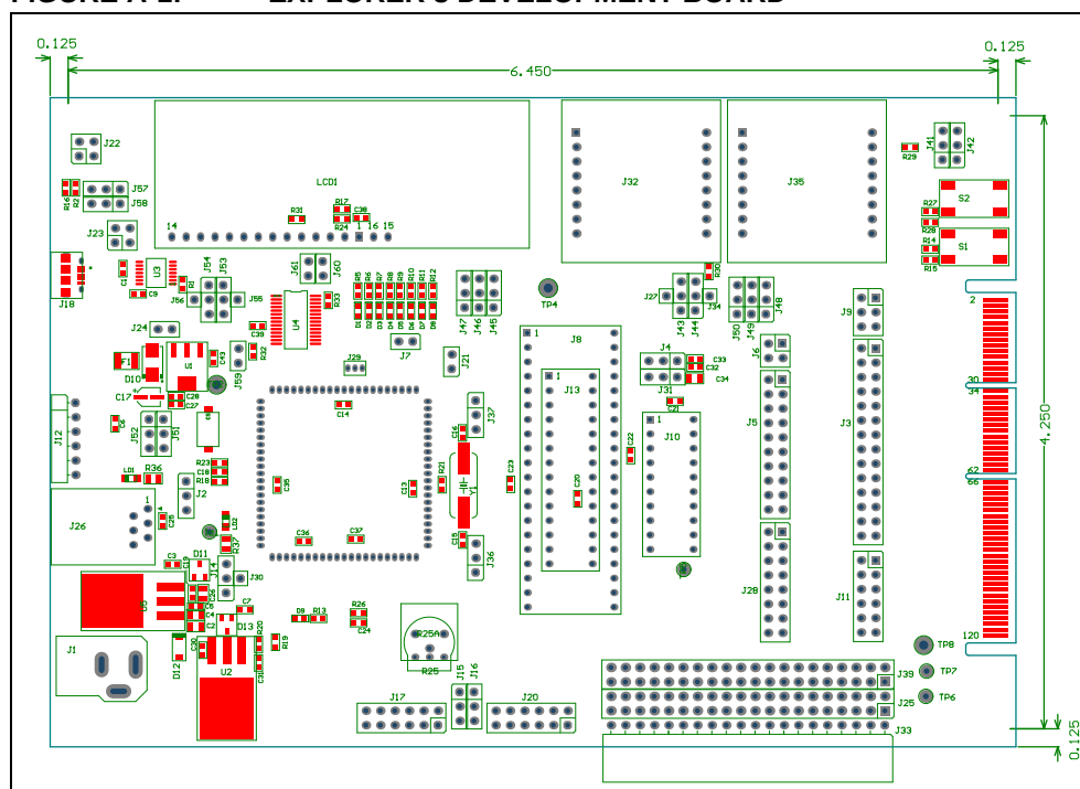
FIGURE A-1: EXPLORER 8 DEVELOPMENT BOARD
