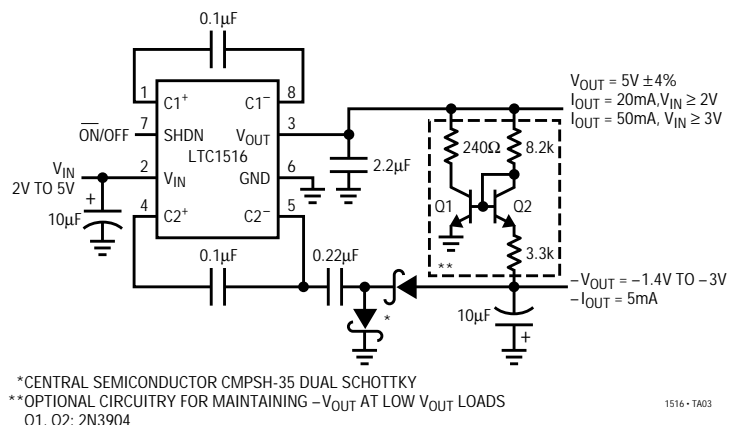
Generating 5V and a Negative Supply
