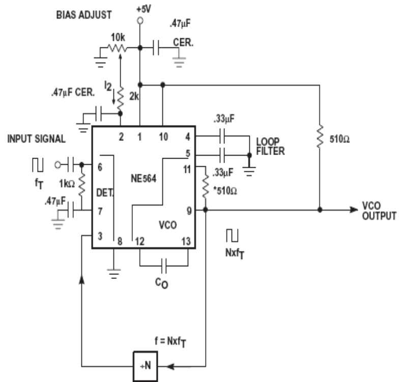
Figure 12. NE564 Phase-Locked Frequency Multiplier
