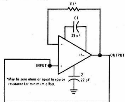
Voltage Follower
