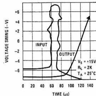
Female Follower Pulse Response
