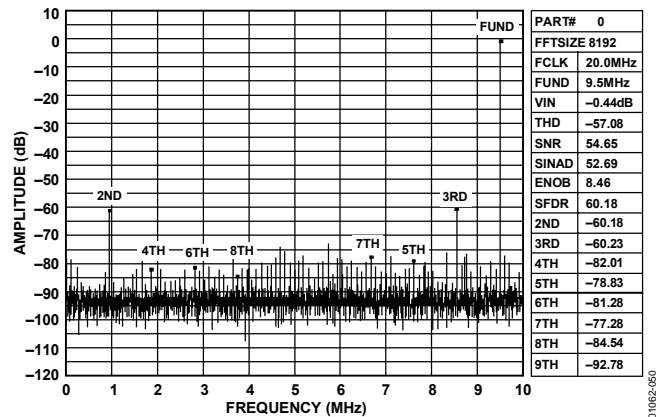
Figure 50. FFT Plot for AD8051 Driving the AD9201 at 9.5 MHz
