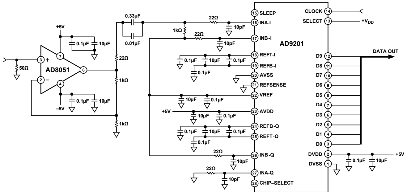
Figure 48. The AD8051 Driving an AD9201, a 10-Bit, 20 MSPS A/D Converter
