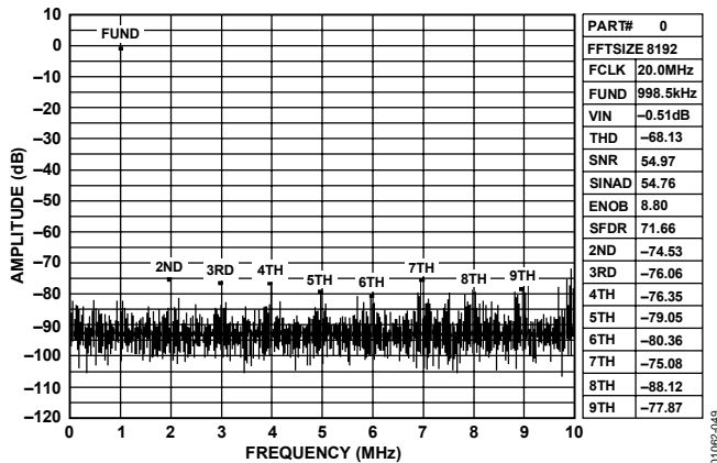
Figure 49. FFT Plot for AD8051 Driving the AD9201 at 1 MHz
