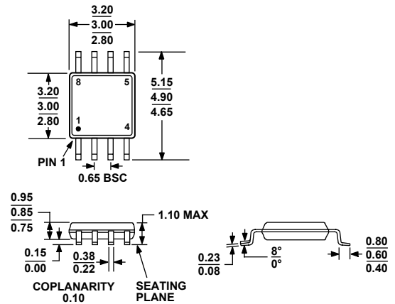
Figure 55. 8-Lead Mini Small Outline Package [MSOP] (RM-8)
