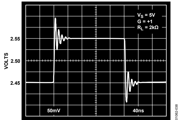
Figure 38. AD8054 100 mV Step Response; V_S = 5\text{V} , G = +1
