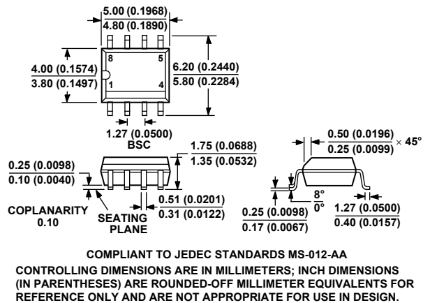
Figure 56. 8-Lead Standard Small Outline Package [SOIC_N] Narrow Body (R-8)
