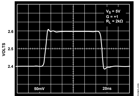
Figure 35. AD8051/AD8052 200 mV Step Response; V_S = 5\text{V} , G = +1
