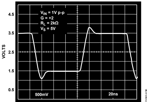
Figure 36. Large Signal Step Response; V_S = 5\text{V} , G = +2
