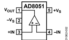
Figure 2. SOT-23-5 (RJ)
