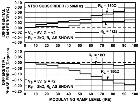
Figure 21. AD8051/AD8052 Differential Gain and Phase Errors
