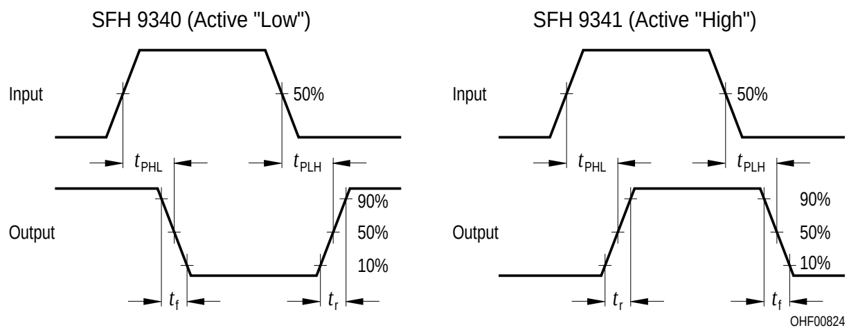
Figure 2 Switching Time Definitions
