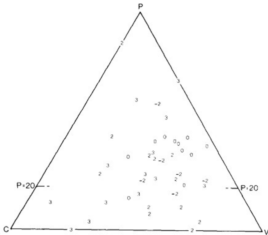
Fig. 1. Ternary diagram of planar ( P ), concave ( C ) and convex ( V ) perimeters of grains from sample SA2. The phi diameter of each grain is plotted.
