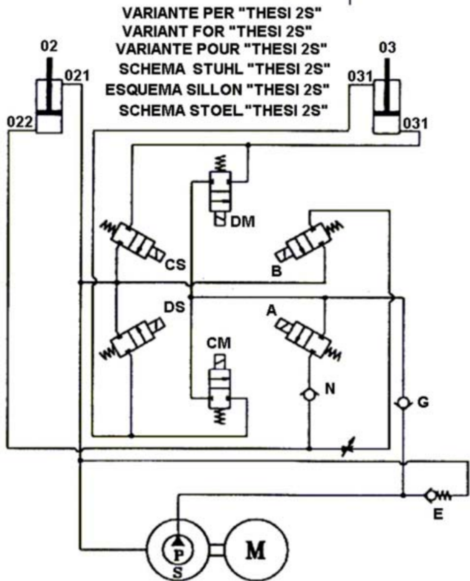
“THESI 2” CHAIR HYDRAULIC DIAGRAM
